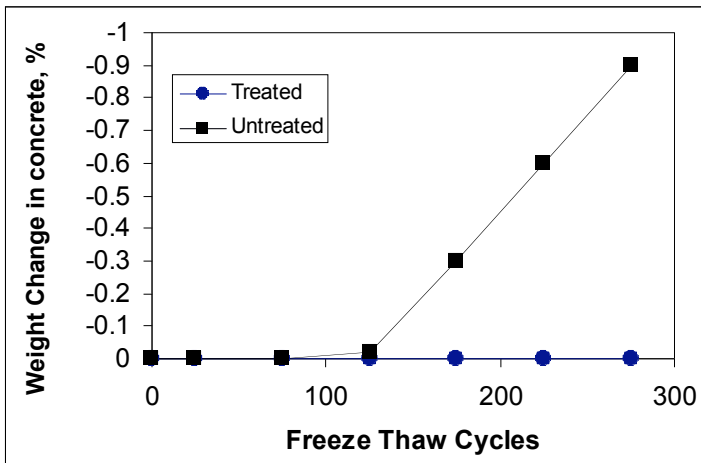
ASTM C-666-97
