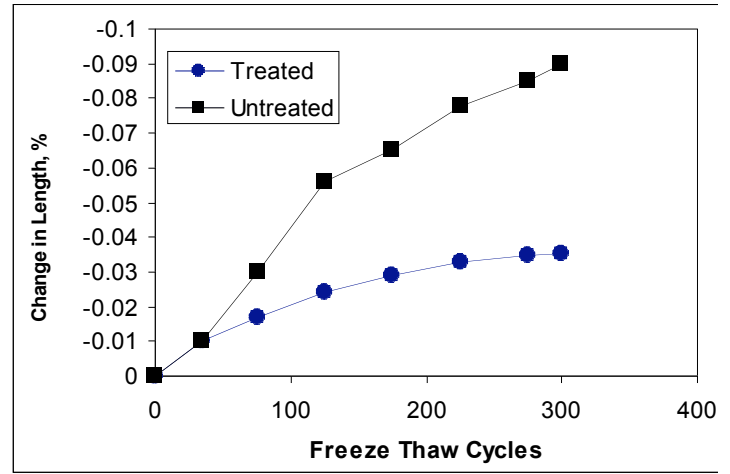
Freezing & Thawing effect on treated & untreated concrete samples ASTM C666-97
